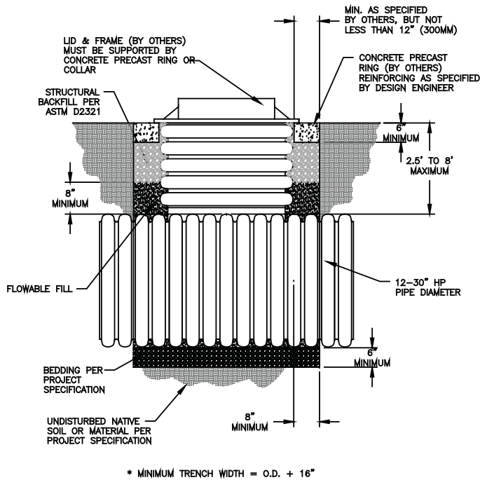
Figure 6: Vertical Riser
