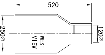
VALVE BOX WITH LARGE BOOT 250 TO 400 VALVE
