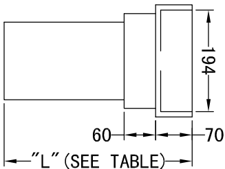
TYPE "A" VALVE BOX RISERS
