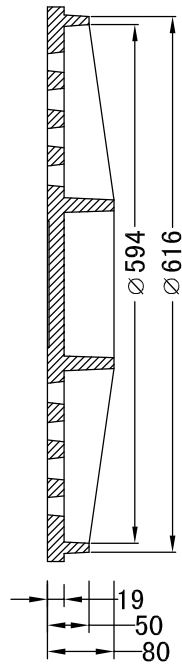
SECTION "A-A"
