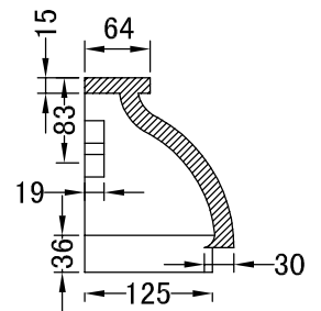
SECTION G-G
