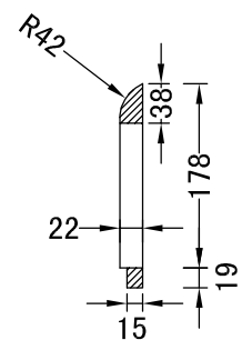
SECTION E-E
