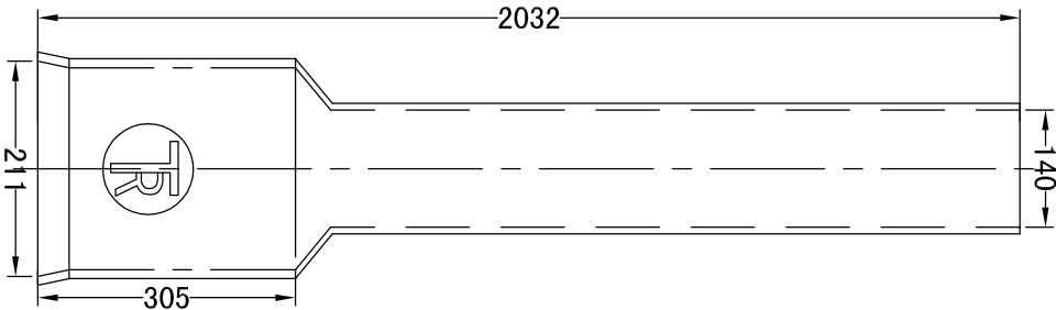
TYPE "A" VALVE BOX BOTTOM CAST IRON
