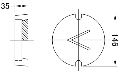
COVER
