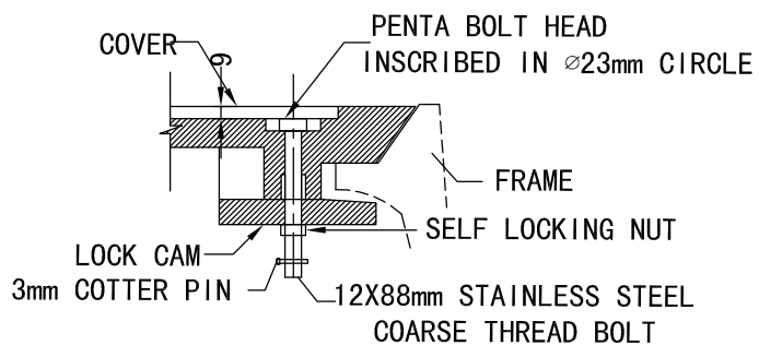
COVER WITH LOCK 2LOCKS PER COVER
