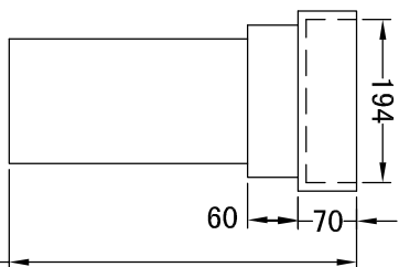
TYPE "A" VALVE BOX RISERS
