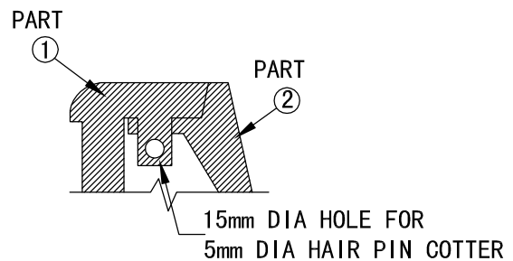
LOCKING DEVICE DETAIL
