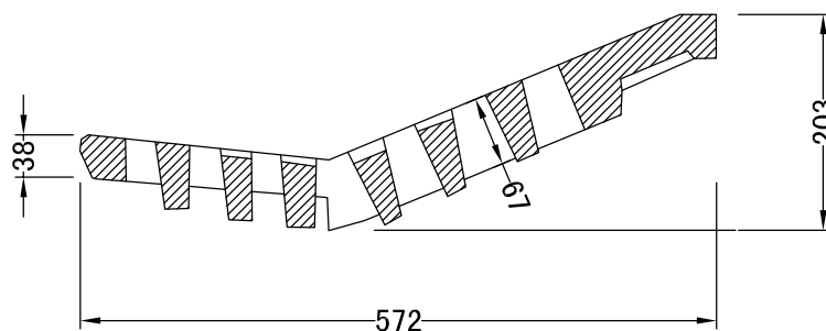
SECTION "A"
