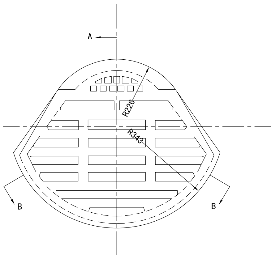
PLAN OF COVER
