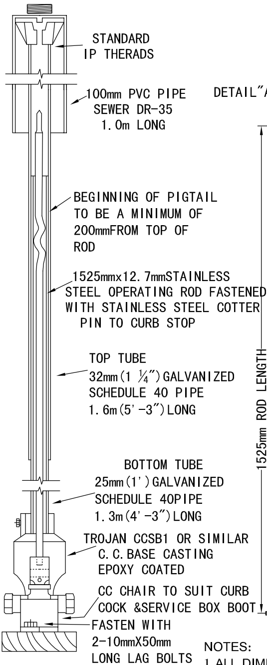
DETAIL A
