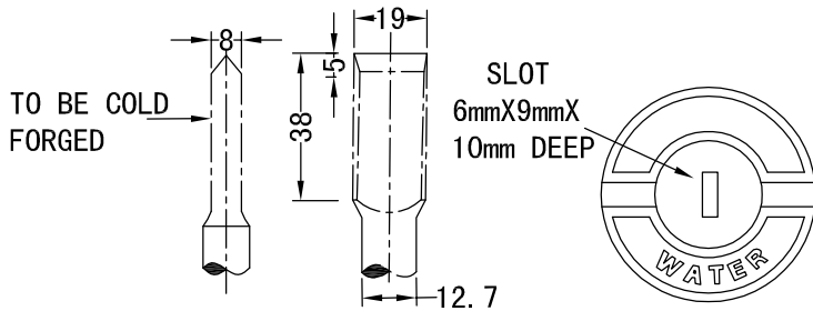
DETAIL A
