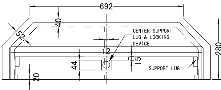
PART ② PLAN
