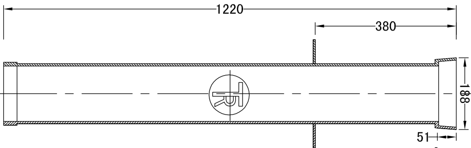
TYPE "A" VALVE BOX TOP CAST IRON
