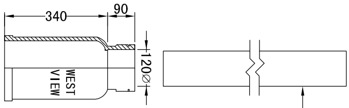
VALVE BOX WITH SMALL BOOT 100 TO 200 VALVE
