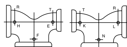
DOUBLE BRANCH ELBOW
