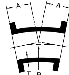
BENDS, 1/16 (22-1/2 DEG)
