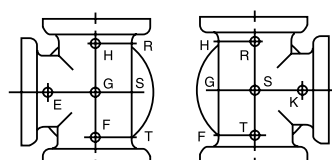
FRONT VIEW SIDE VIEW SIDE OUTLET TEE STRAIGHT SIZE
