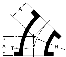
BENDS, 1/8 (45 DEG)
