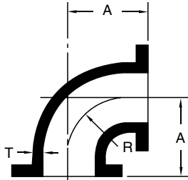
BENDS, 1/4 (90 DEG)
