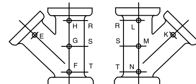
45° LATERAL STRAIGHT SIZE
