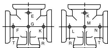
BASE TEE
