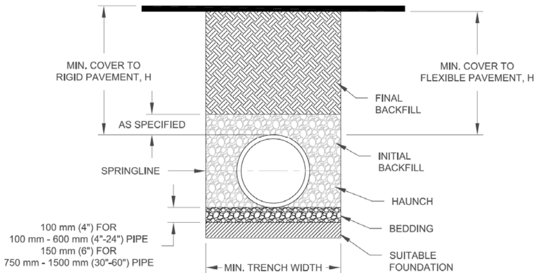
Figure 1 ADS SaniTite HP Pipe (CSA B182.13) Trench Detail Under Pavement
